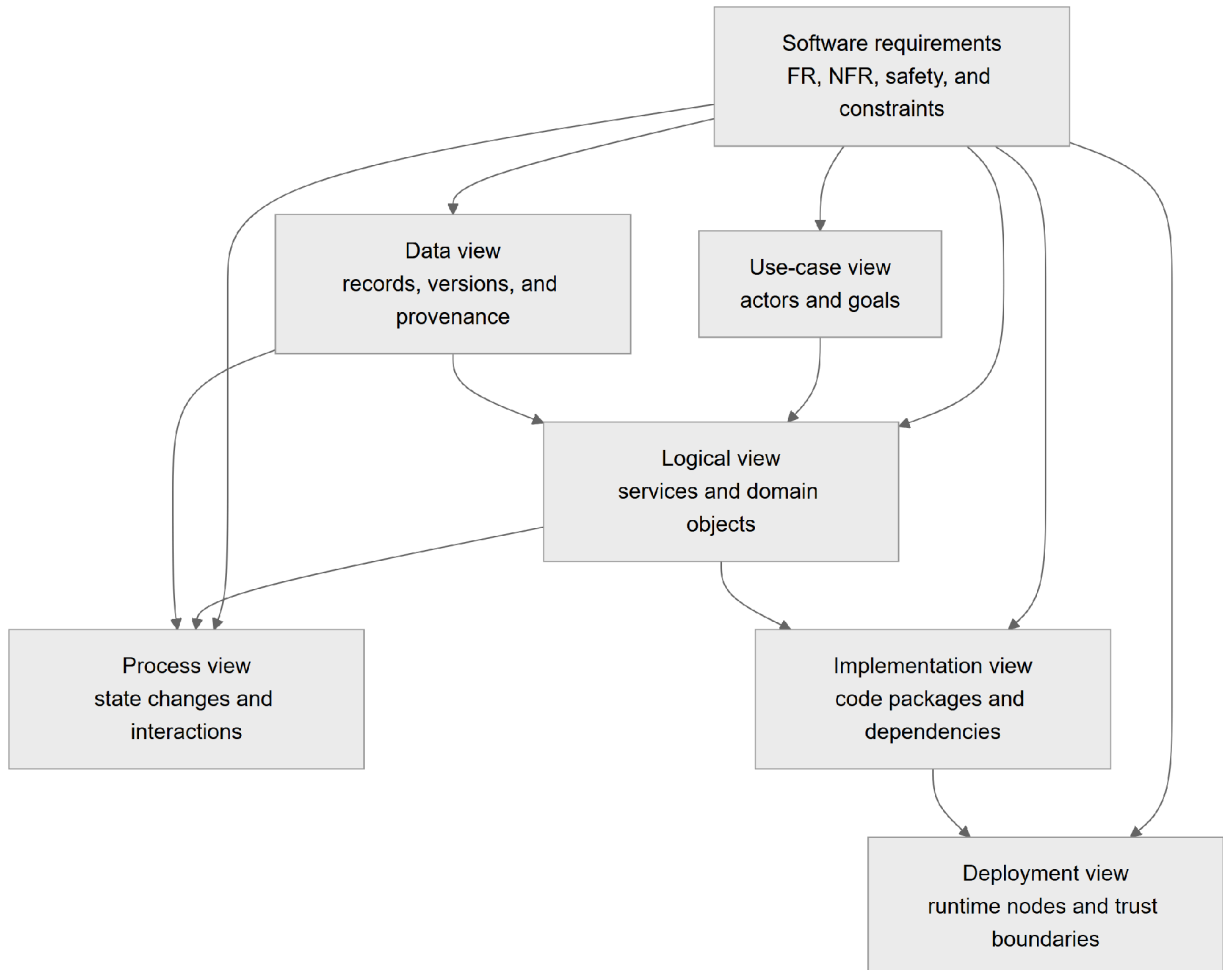
Figure 1. Architectural views and their relationships.
