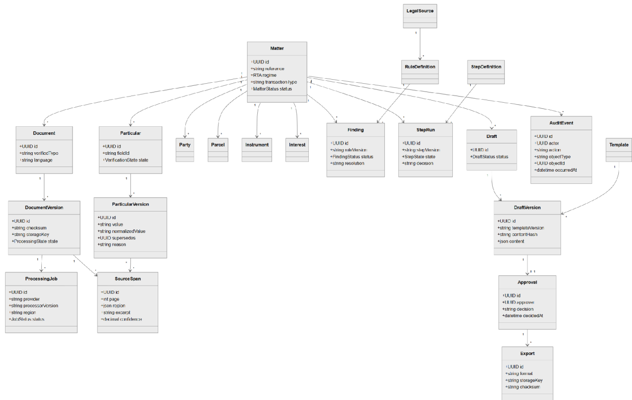
Figure 5. Significant domain classes and provenance relationships.
