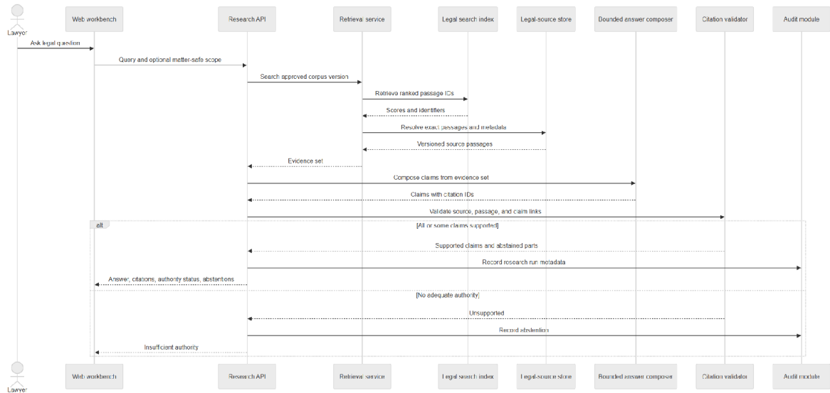
Figure 8. Grounded legal-research sequence.
