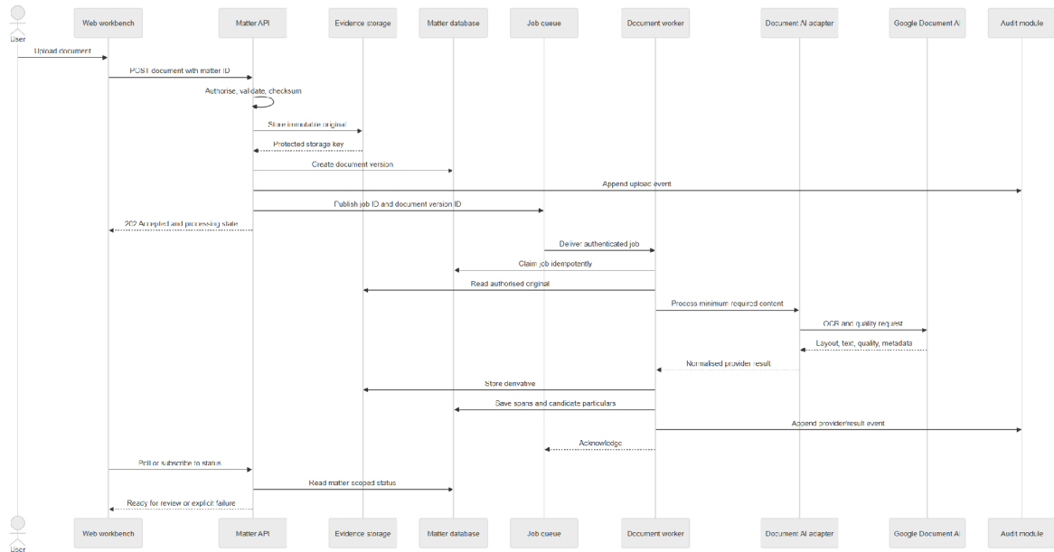
Figure 7. Internal sequence for asynchronous document processing.
